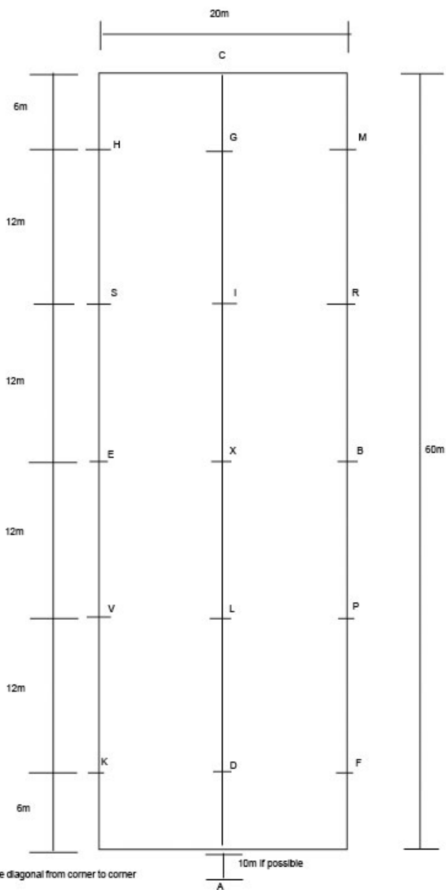
DIAGRAM OF 20 x 60m ARENA
